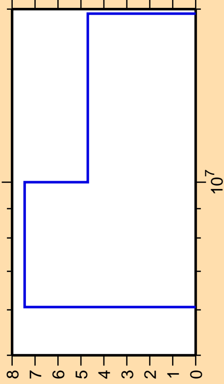
\Delta\sigma/\sigma vs. E for ^{183}\text{Re}(n,2n)
