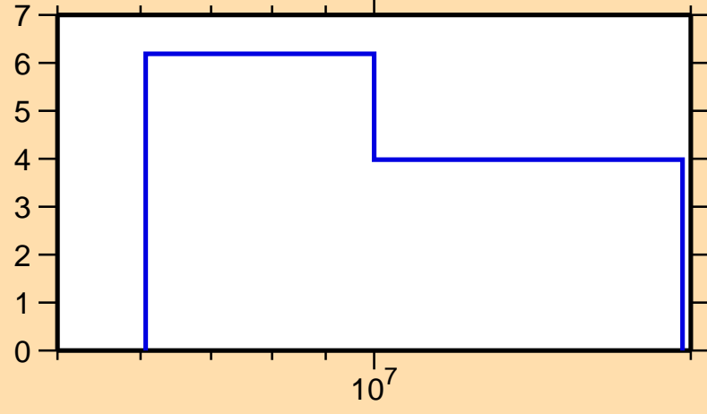
\Delta\sigma/\sigma vs. E for ^{183}\text{Re}(n,\text{el.})
