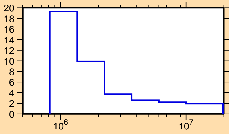
\Delta\sigma/\sigma vs. E for ^{183}\text{Re}(n,n\text{onel.})
