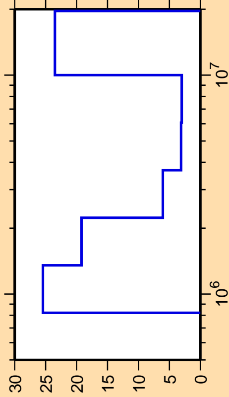
\Delta\sigma/\sigma vs. E for ^{183}\text{Re}(n,n\text{cont.})
