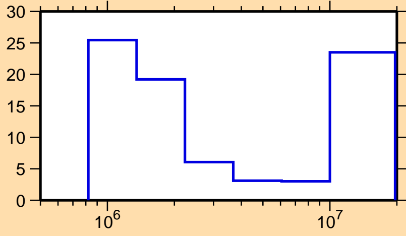
\Delta\sigma/\sigma vs. E for ^{183}\text{Re}(n,n\text{cont.})
