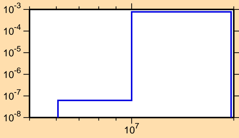
\sigma vs. E for ^{183}\text{Re}(n,d)
