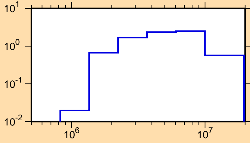
\sigma vs. E for ^{183}\text{Re}(n,n\text{cont.})
