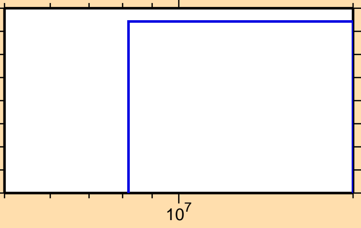
\sigma vs. E for ^{183}\text{Re}(n,2n\alpha)
