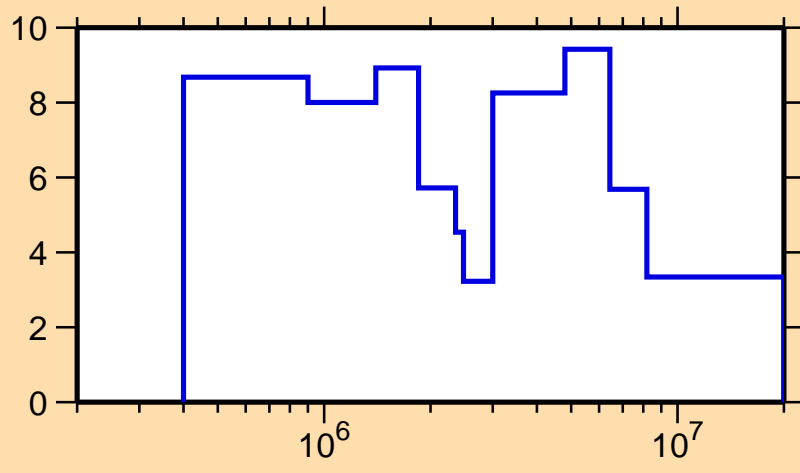
\Delta\sigma/\sigma vs. E for ^{183}\text{Re}(n,el.)
