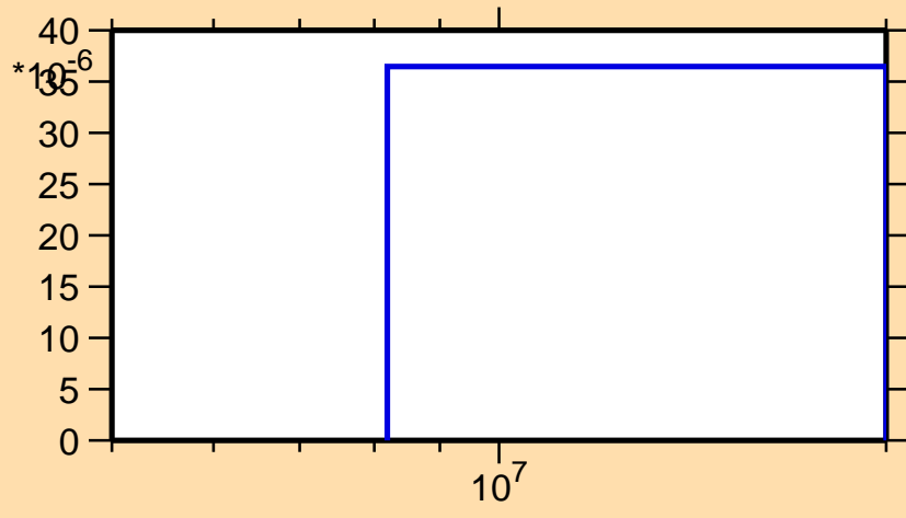
\sigma vs. E for ^{183}\text{Re}(n,t)
