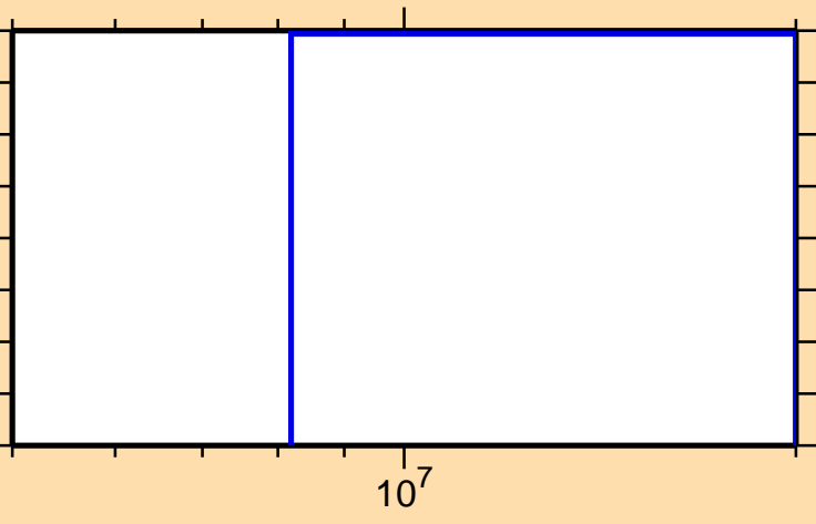
\sigma vs. E for ^{183}\text{Re}(\text{mt } 42)
