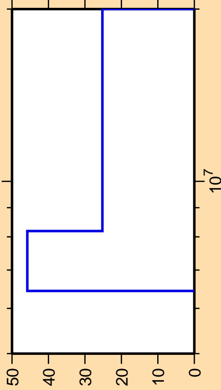
\Delta\sigma/\sigma vs. E for ^{184}\text{Re}(n,np)
