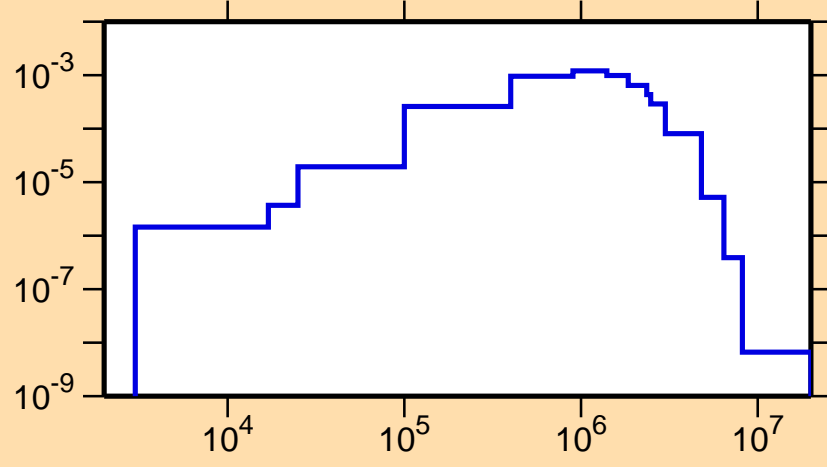
\sigma vs. E for ^{184}\text{Re}(n,n_1)
