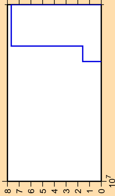
\Delta\sigma/\sigma vs. E for ^{185}\text{Re}(n,p\alpha)
