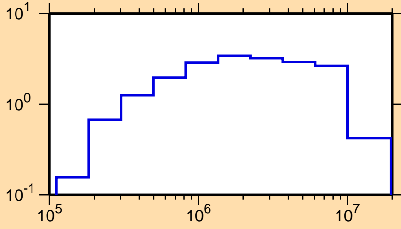
\sigma vs. E for ^{185}\text{Re}(n,\text{inel.})
