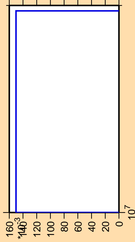
\Delta\sigma/\sigma vs. E for ^{185}\text{Re}(n,p\alpha)
