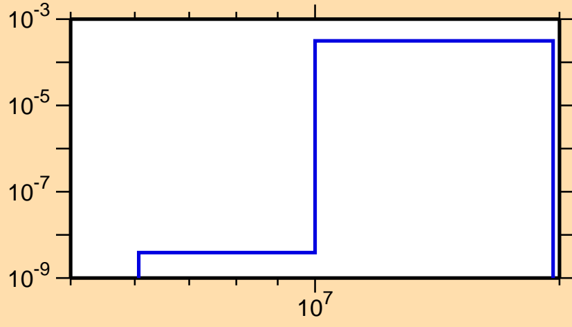
\sigma vs. E for ^{185}\text{Re}(n,np)
