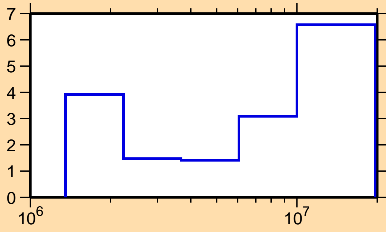
\Delta\sigma/\sigma vs. E for ^{185}\text{Re}(n,\text{inel.})
