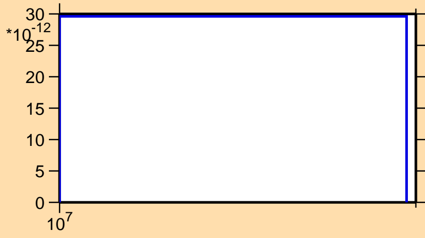
\sigma vs. E for ^{185}\text{Re}(n,\text{He}3)
