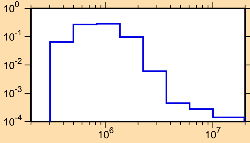
\sigma vs. E for ^{185}\text{Re}(n,n_3)
