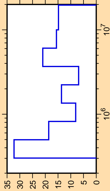
\Delta\sigma/\sigma vs. E for ^{185}\text{Re}(n,n_3)
