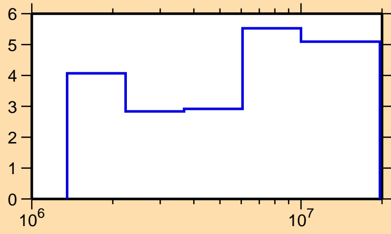
\Delta\sigma/\sigma vs. E for ^{185}\text{Re}(n,n\text{cont.})
