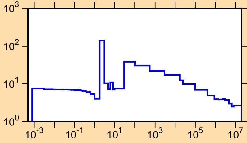
\sigma vs. E for ^{185}\text{Re}(n,\text{el.})
