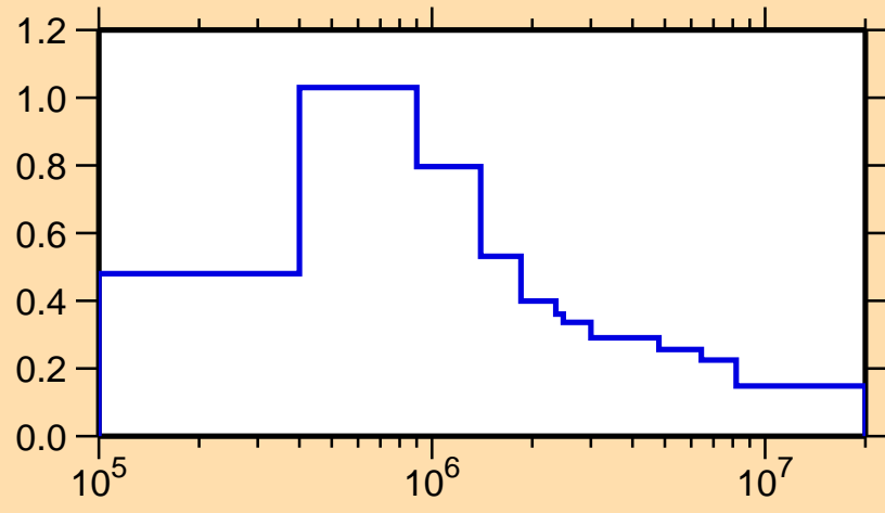
\sigma vs. E for ^{185}\text{Re}(n,n_1)
