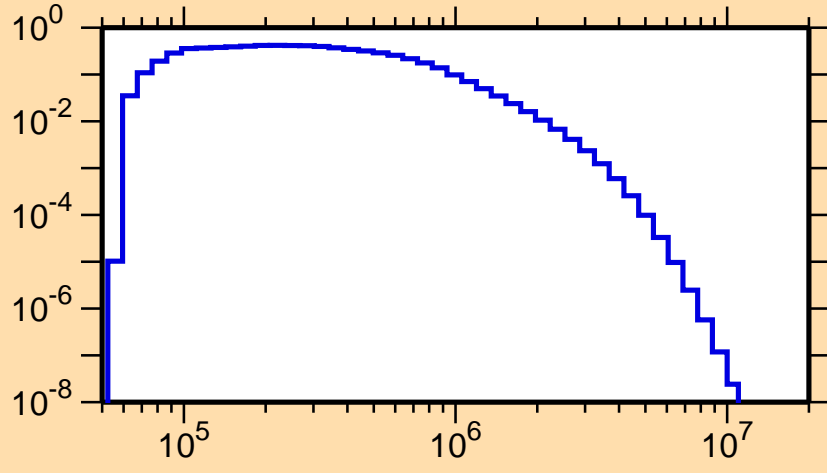
\sigma vs. E for ^{186}\text{Re}(n,n_1)
