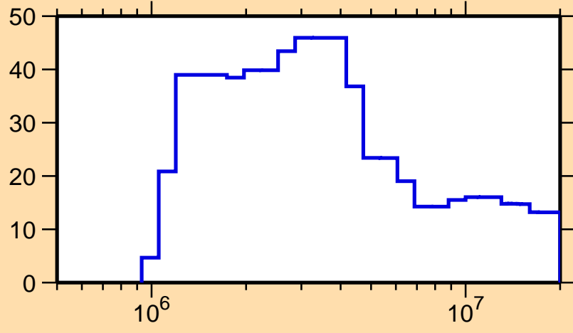
\Delta\sigma/\sigma vs. E for ^{186}\text{Re}(n,p)
