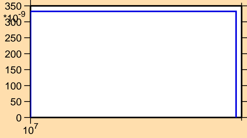
\sigma vs. E for ^{186}\text{Re}(n,nd)
