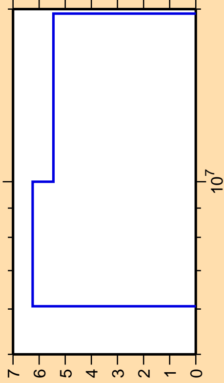
\Delta\sigma/\sigma vs. E for ^{186}\text{Re}(n,2n)
