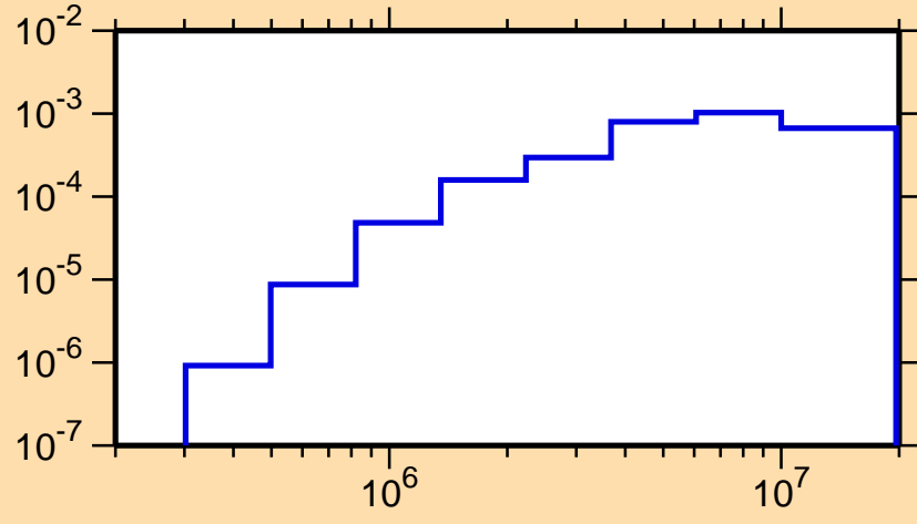
\sigma vs. E for ^{186}\text{Re}(n,n_4)
