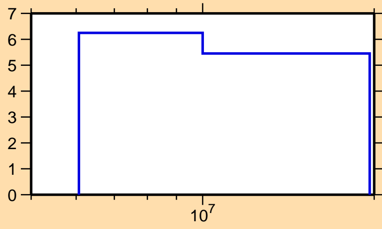
\Delta\sigma/\sigma vs. E for ^{186}\text{Re}(n,2n)
