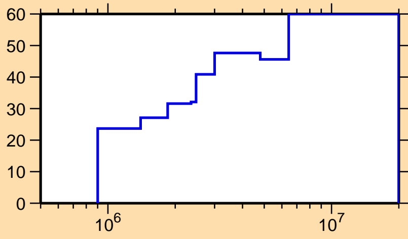
\Delta\sigma/\sigma vs. E for ^{186}\text{Re}(n,n_1)
