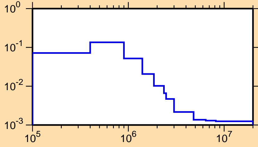
\sigma vs. E for ^{186}\text{Re}(n,n_3)
