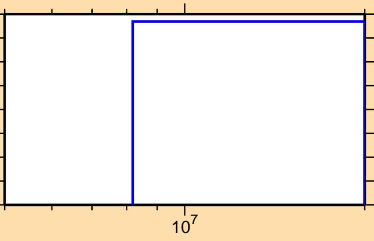
\sigma vs. E for ^{186}\text{Re}(n,2np)
