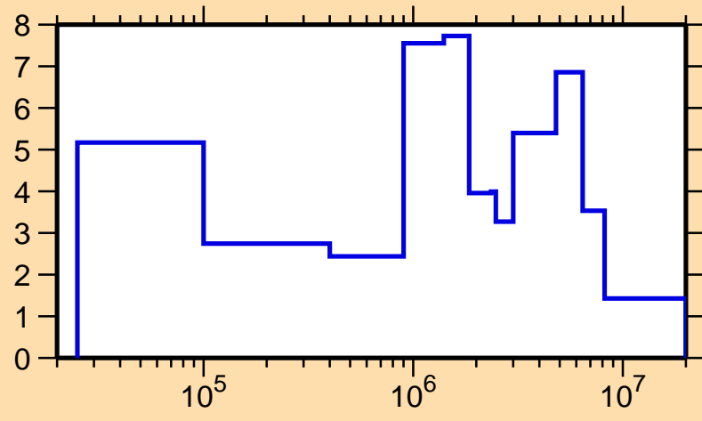
\Delta\sigma/\sigma vs. E for ^{186}\text{Re}(n,\text{el.})
