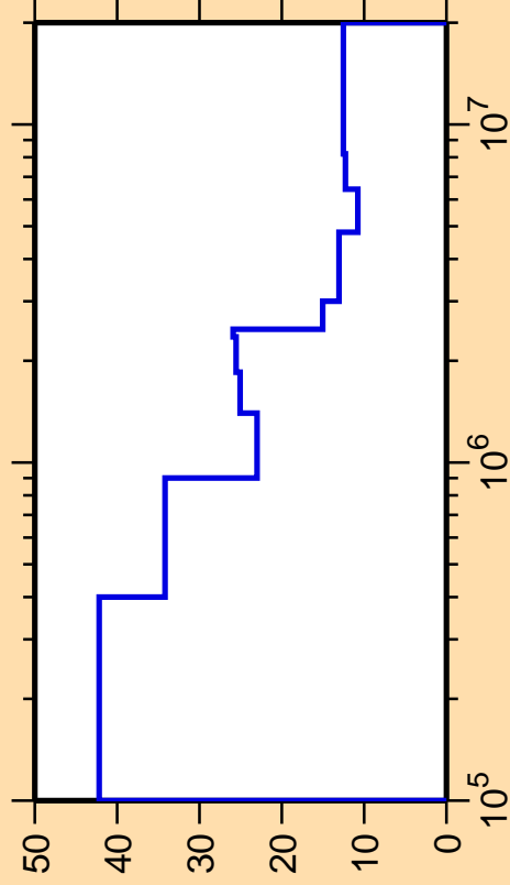
\Delta\sigma/\sigma vs. E for ^{186}\text{Re}(n,n_2)
