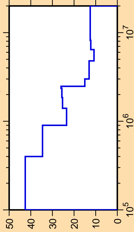
\Delta\sigma/\sigma vs. E for ^{186}\text{Re}(n,n_3)
