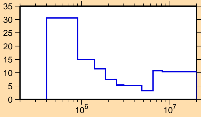
\Delta\sigma/\sigma vs. E for ^{186}\text{Re}(n,n\text{cont.})
