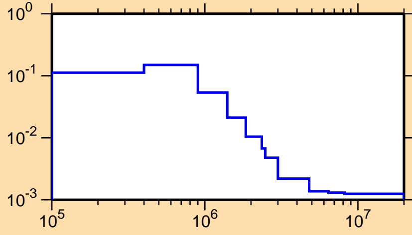
\sigma vs. E for ^{186}\text{Re}(n,n_2)
