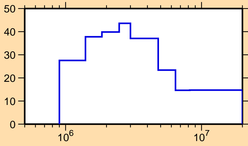
\Delta\sigma/\sigma vs. E for ^{186}\text{Re}(n,p)
