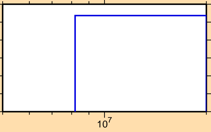
\sigma vs. E for ^{186}\text{Re}(n,2np)
