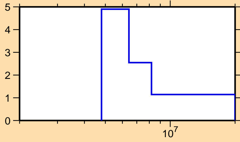
\Delta\sigma/\sigma vs. E for ^{186}\text{Re}(n,\text{tot.})
