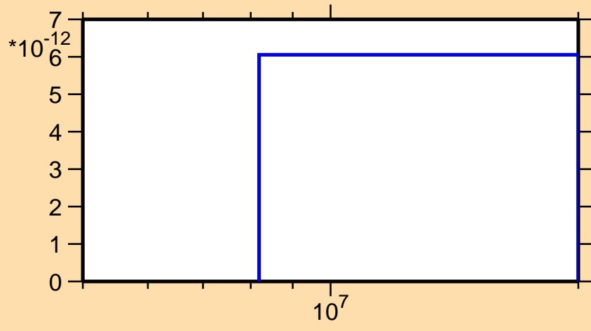
\sigma vs. E for ^{186}\text{Re}(n,\text{He}3)
