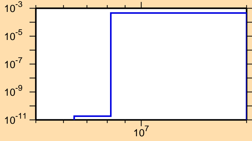
\sigma vs. E for ^{186}\text{Re}(n,d)
