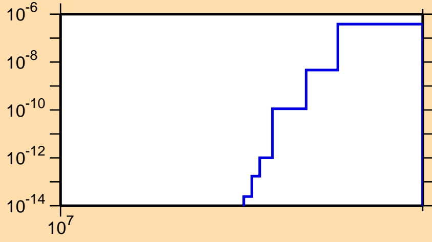
\sigma vs. E for ^{187}\text{Re}(n,nt)
