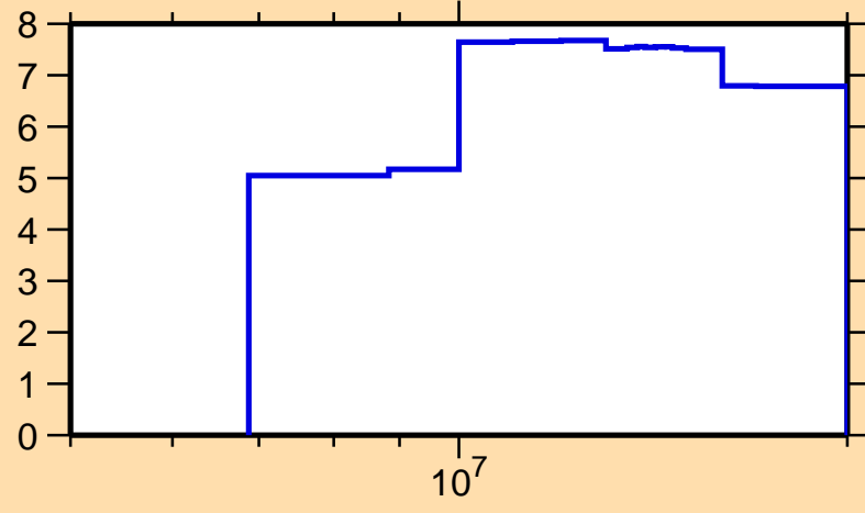
\Delta\sigma/\sigma vs. E for ^{187}\text{Re}(n,\text{inel.})
