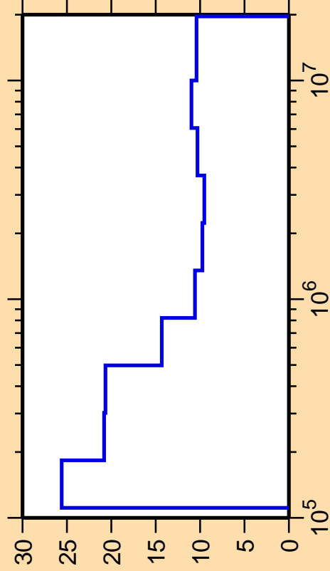
\Delta\sigma/\sigma vs. E for ^{187}\text{Re}(n,n_1)
