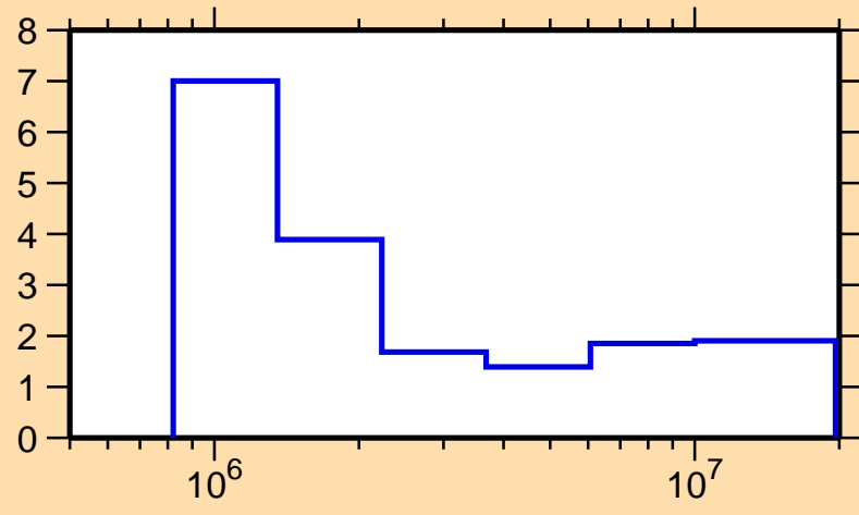
\Delta\sigma/\sigma vs. E for ^{187}\text{Re}(n,n\text{onel.})
