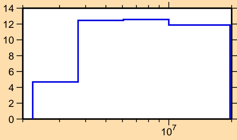
\Delta\sigma/\sigma vs. E for ^{187}\text{Re}(n,p)
