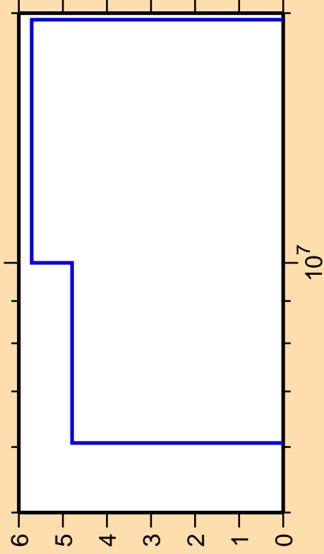
\Delta\sigma/\sigma vs. E for ^{187}\text{Re}(n,2n)
