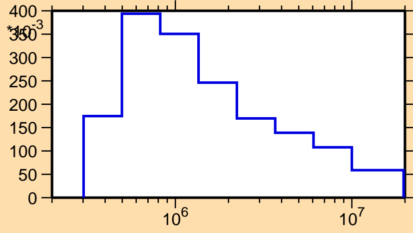
\sigma vs. E for ^{187}\text{Re}(n,n_3)
