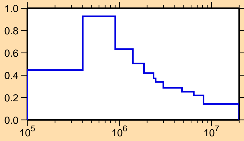
\sigma vs. E for ^{187}\text{Re}(n,n_1)
