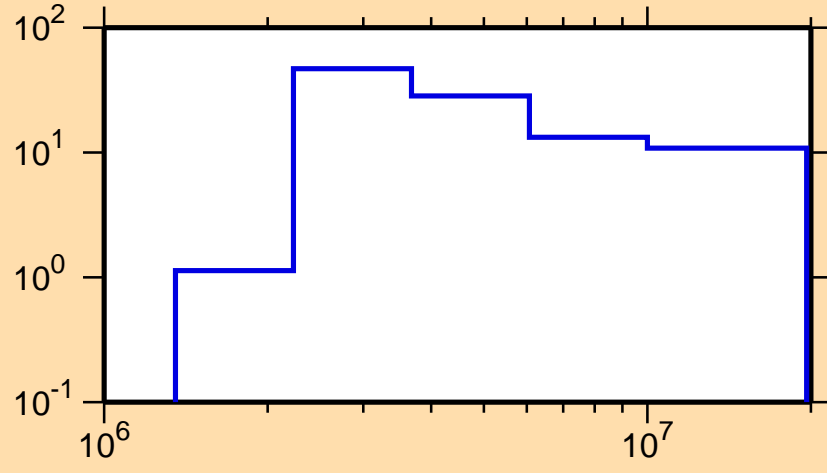
\Delta\sigma/\sigma vs. E for ^{188}\text{Re}(n,p)
