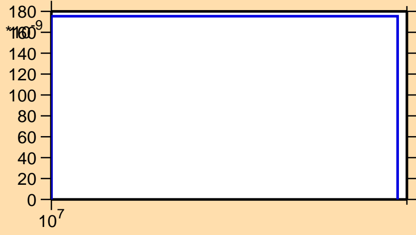
\sigma vs. E for ^{188}\text{Re}(n,nd)
