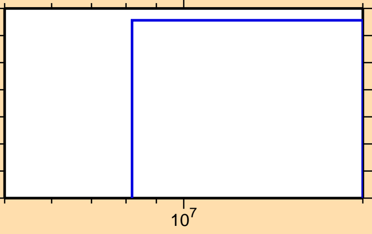
\sigma vs. E for ^{188}\text{Re}(n,2n\alpha)
