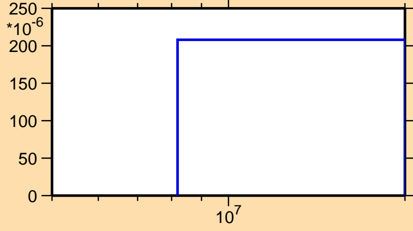
\sigma vs. E for ^{188}\text{Re}(n,np)
