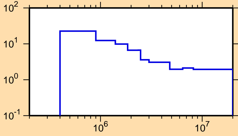
\Delta\sigma/\sigma vs. E for ^{188}\text{Re}(n,n\text{onel.})
