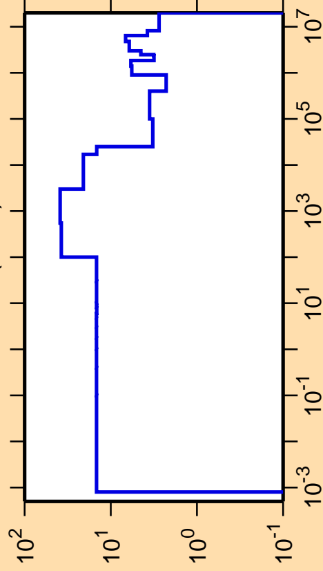
\Delta\sigma/\sigma vs. E for ^{188}\text{Re}(n,\text{el.})
