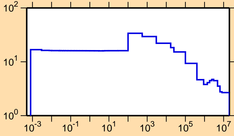
\sigma vs. E for ^{188}\text{Re}(n,\text{el.})
