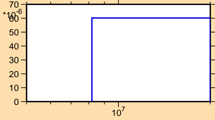
\sigma vs. E for ^{188}\text{Re}(n,t)
