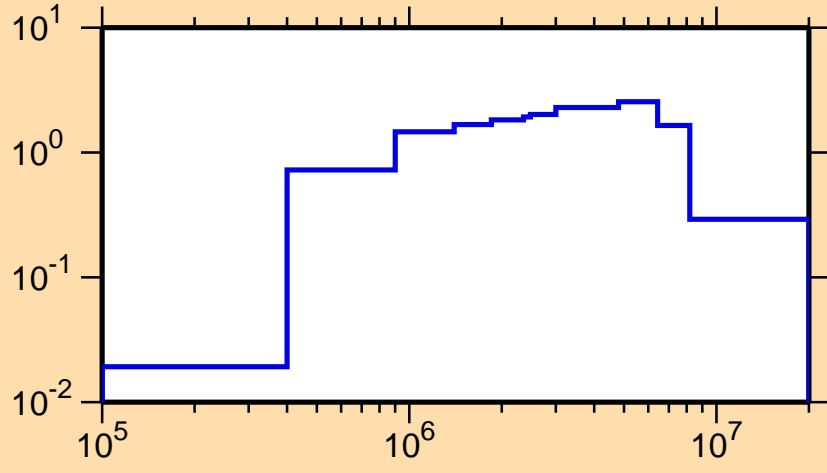
\sigma vs. E for ^{188}\text{Re}(n,n\text{cont.})
