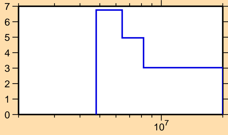
\Delta\sigma/\sigma vs. E for ^{188}\text{Re}(n,2n)
