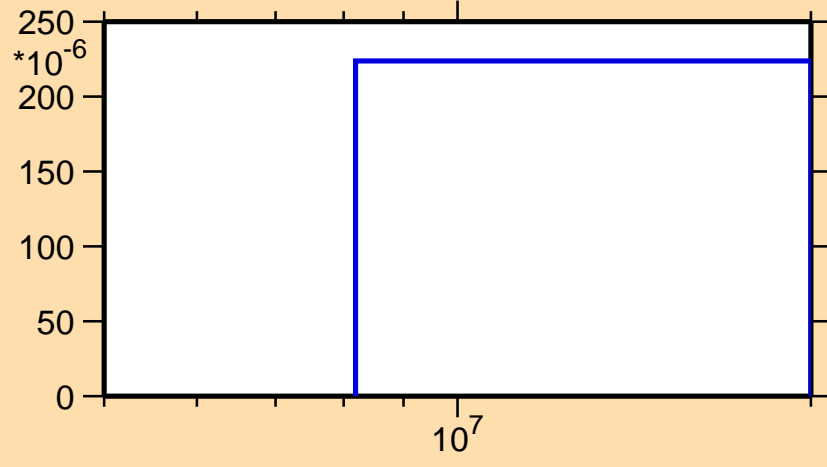
\sigma vs. E for ^{188}\text{Re}(n,np)
