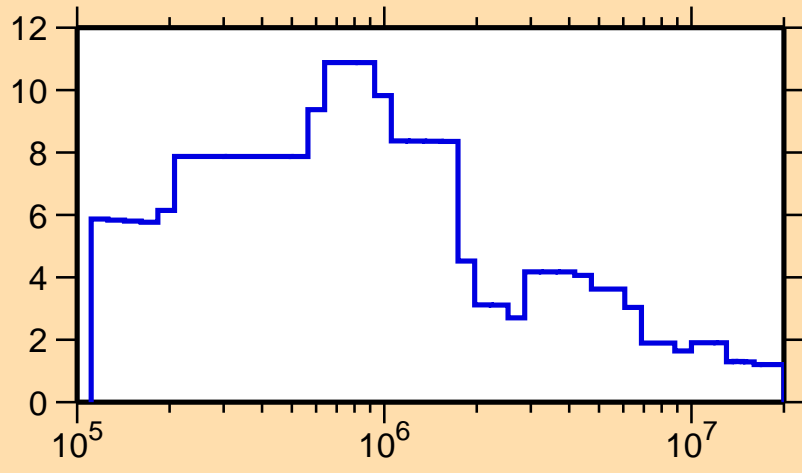
\Delta\sigma/\sigma vs. E for ^{189}\text{Re}(n,\text{tot.})
