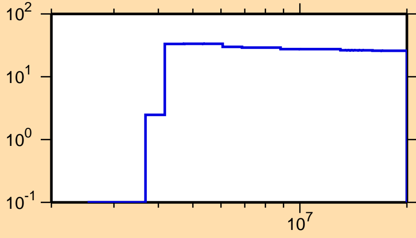
\Delta\sigma/\sigma vs. E for ^{189}\text{Re}(n,p)
