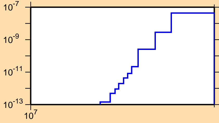
\sigma vs. E for ^{189}\text{Re}(n,2n\alpha)
