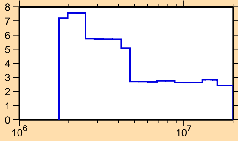
\Delta\sigma/\sigma vs. E for ^{189}\text{Re}(n,\text{nonel.})
