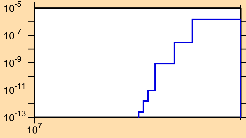
\sigma vs. E for ^{189}\text{Re}(n,nt)
