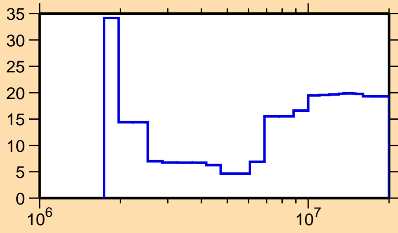
\Delta\sigma/\sigma vs. E for ^{189}\text{Re}(n,n\text{cont.})
