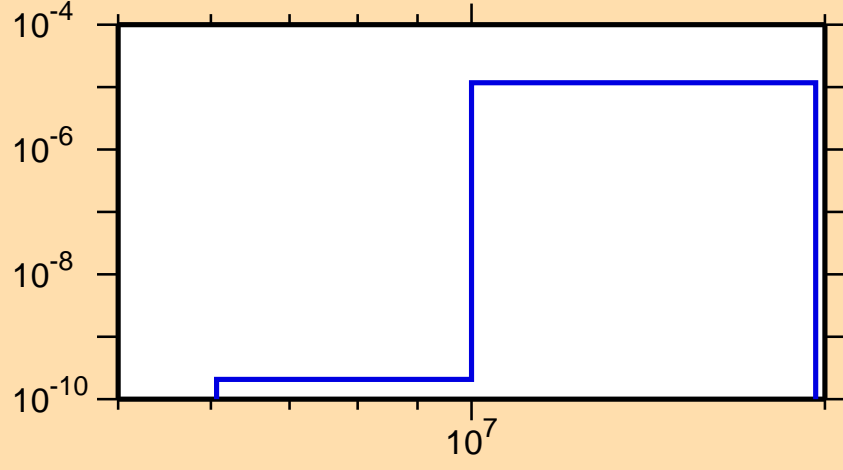
\sigma vs. E for ^{189}\text{Re}(n,n\alpha)
