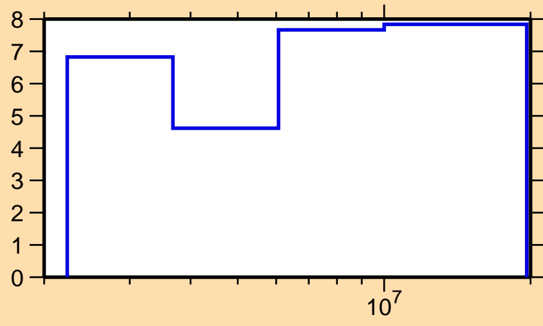
\Delta\sigma/\sigma vs. E for ^{189}\text{Re}(n,\text{inel.})
