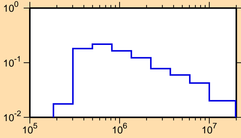
\sigma vs. E for ^{189}\text{Re}(n,n_3)
