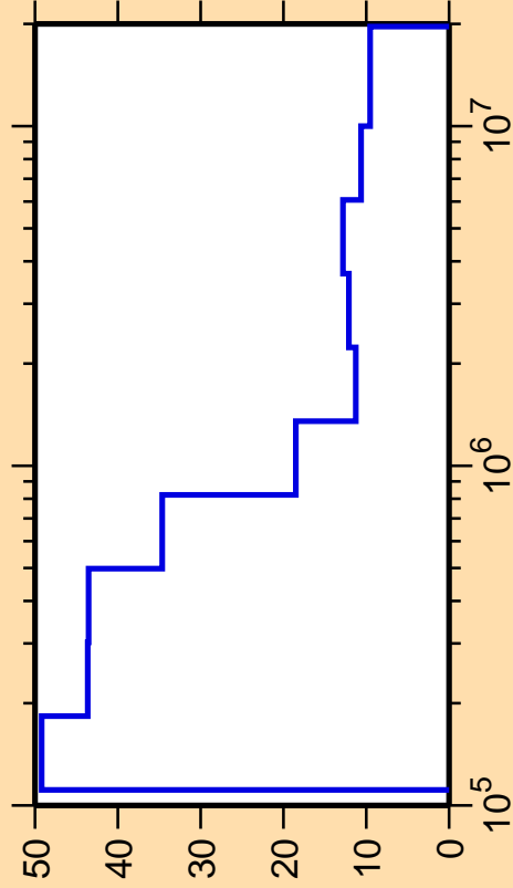
\Delta\sigma/\sigma vs. E for ^{189}\text{Re}(n,n_2)
