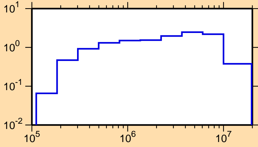
\sigma vs. E for ^{189}\text{Re}(n,\text{inel.})
