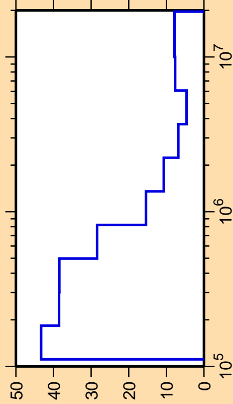
\Delta\sigma/\sigma vs. E for ^{189}\text{Re}(n,\text{inel.})
