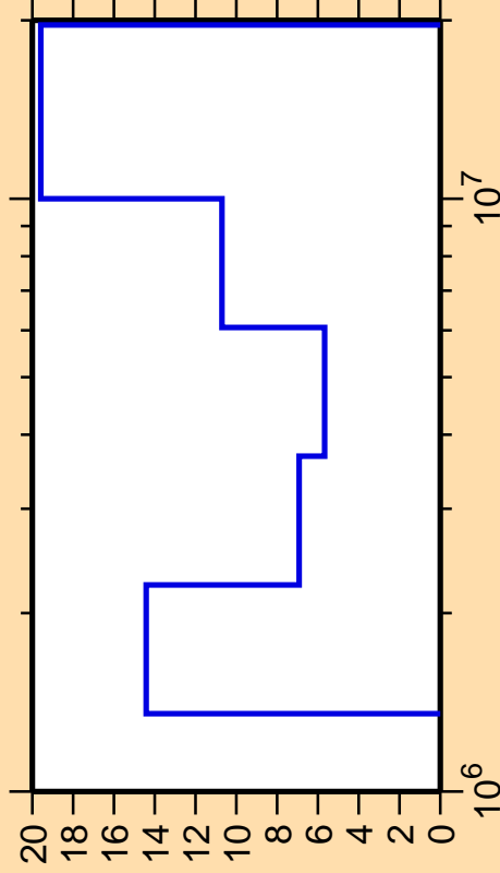
\Delta\sigma/\sigma vs. E for ^{189}\text{Re}(n,n\text{cont.})
