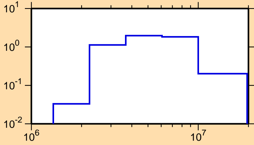
\sigma vs. E for ^{189}\text{Re}(n,n\text{cont.})
