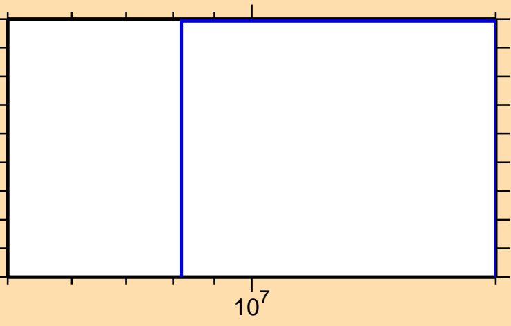
\sigma vs. E for ^{189}\text{Re}(n,t)
