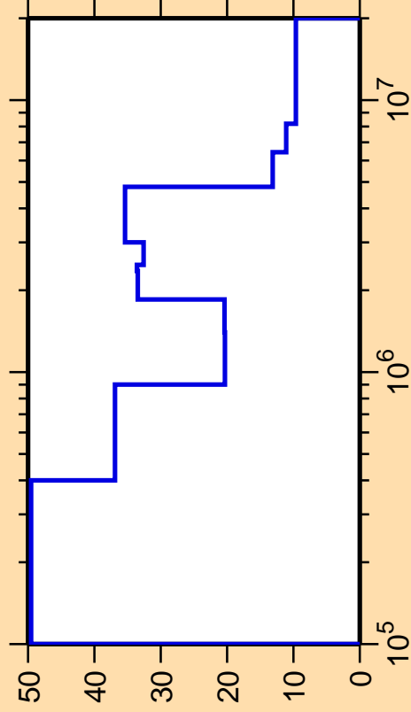
\Delta\sigma/\sigma vs. E for ^{189}\text{Re}(n,n_4)
