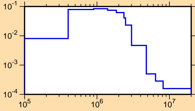
\sigma vs. E for ^{189}\text{Re}(n,n_4)
