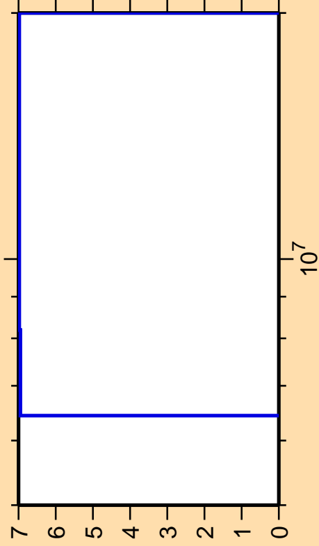
\Delta\sigma/\sigma vs. E for ^{189}\text{Re}(n,2n)
