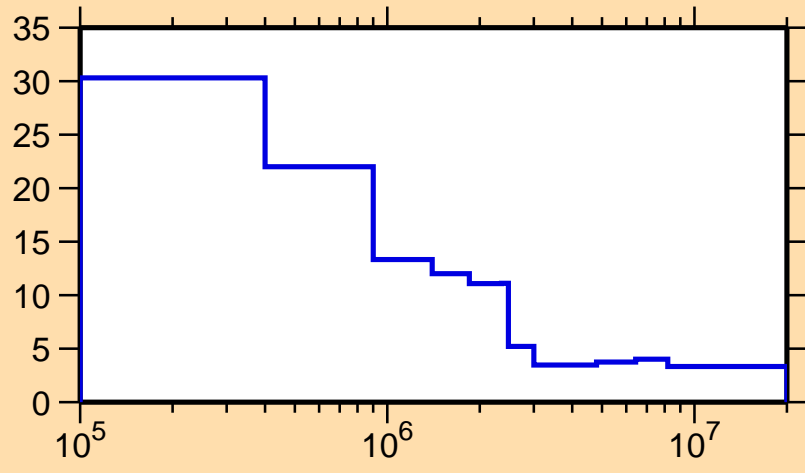
\Delta\sigma/\sigma vs. E for ^{190}\text{Re}(n,n\text{nonel.})
