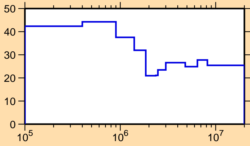
\Delta\sigma/\sigma vs. E for ^{190}\text{Re}(n,n_1)
