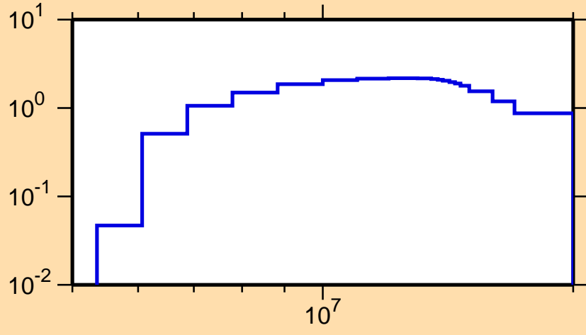
\sigma vs. E for ^{190}\text{Re}(n,2n)
