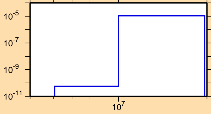
\sigma vs. E for ^{190}\text{Re}(n,n\alpha)
