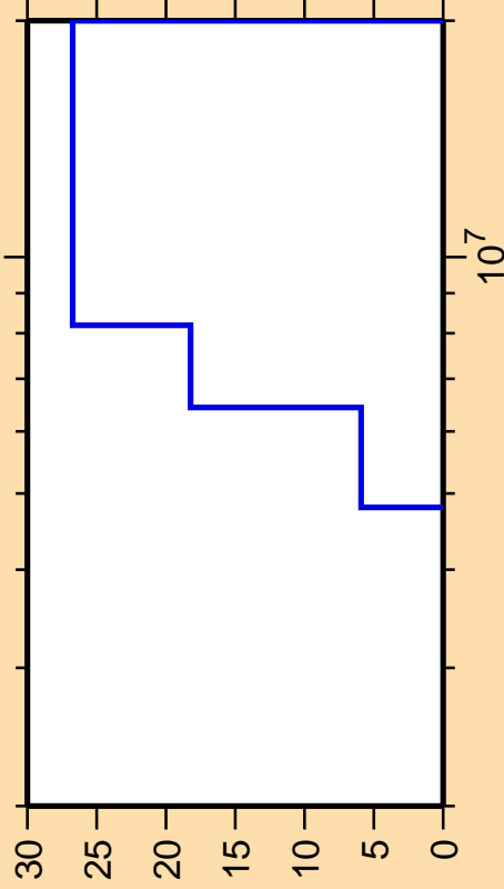
\Delta\sigma/\sigma vs. E for ^{190}\text{Re}(n,n\text{cont.})
