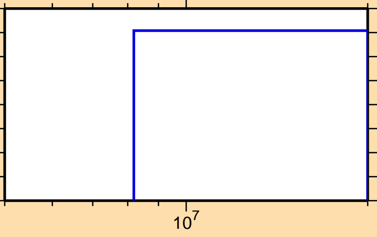
\sigma vs. E for ^{190}\text{Re}(n,t)
