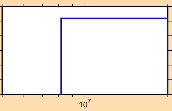
\sigma vs. E for ^{190}\text{Re}(n,2np)
