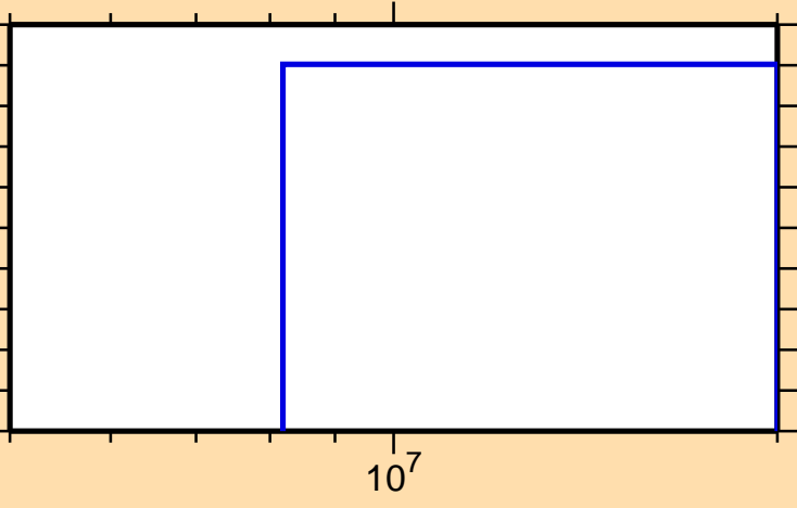
\sigma vs. E for ^{192}\text{Re}(n,n\alpha)
