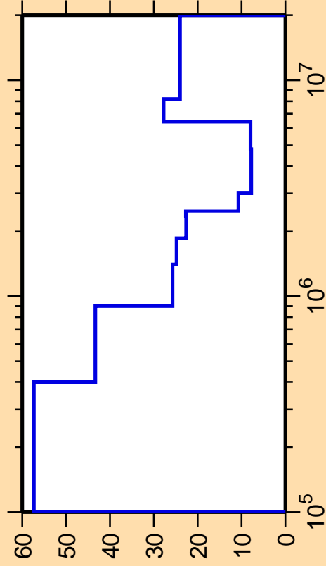
\Delta\sigma/\sigma vs. E for ^{192}\text{Re}(n,\text{inel.})
