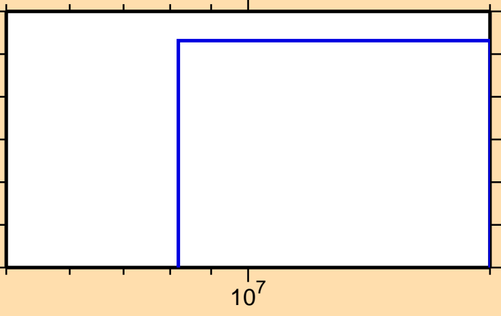
\sigma vs. E for ^{192}\text{Re}(n,d)
