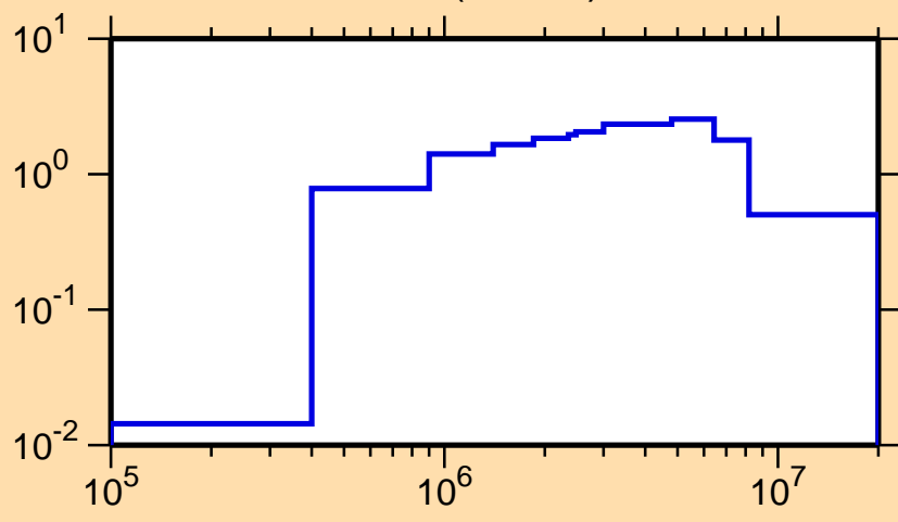
\sigma vs. E for ^{192}\text{Re}(n,\text{inel.})
