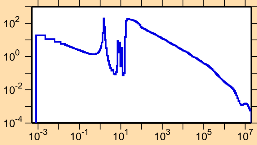
\sigma vs. E for ^{192}\text{Re}(n,\gamma)
