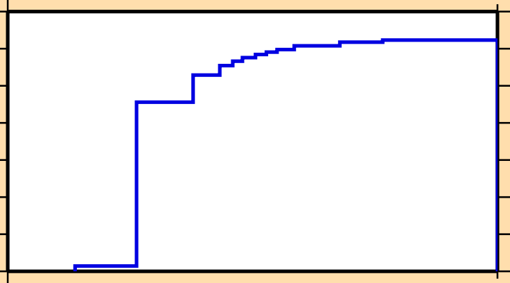
\sigma vs. E for ^{192}\text{Re}(n,3n)
