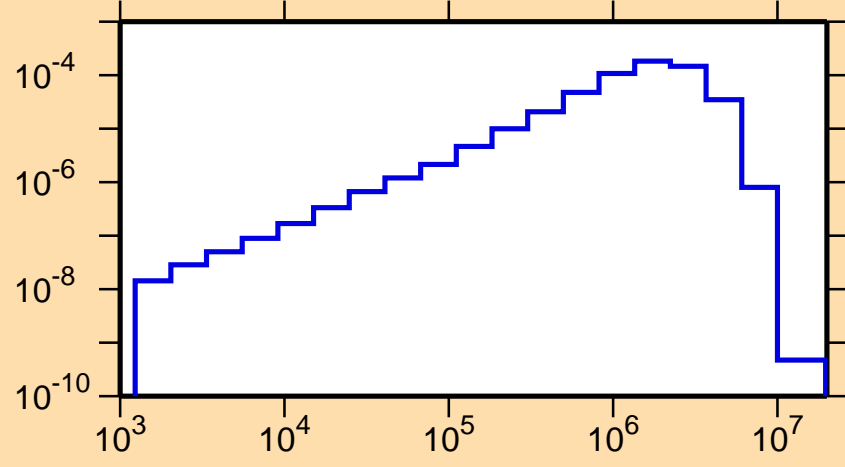
\sigma vs. E for ^{192}\text{Re}(n,n_1)
