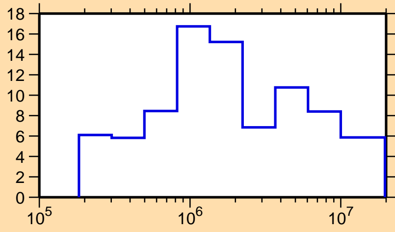
\Delta\sigma/\sigma vs. E for ^{192}\text{Re}(n, el.)
