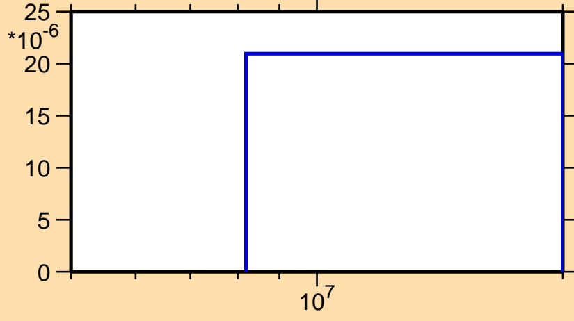
\sigma vs. E for ^{192}\text{Re}(n,t)
