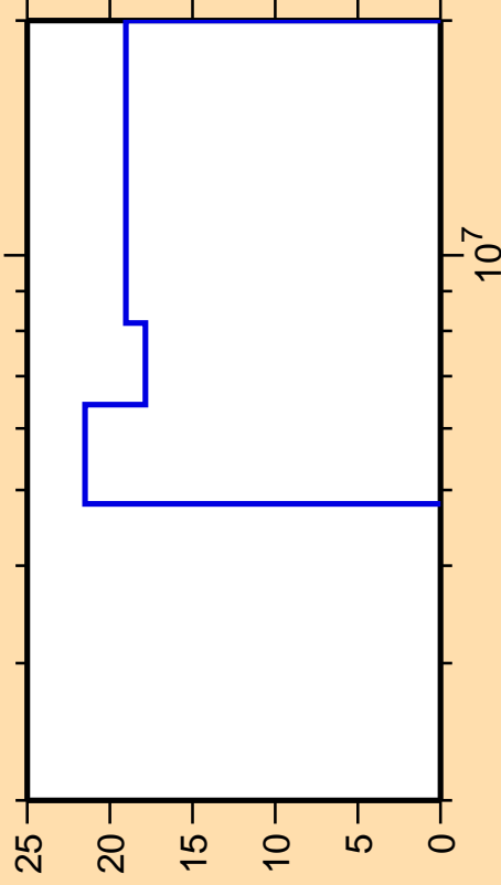
\Delta\sigma/\sigma vs. E for ^{192}\text{Re}(n,n\text{cont.})
