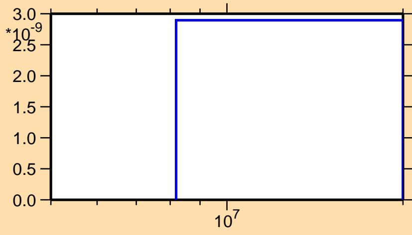
\sigma vs. E for ^{192}\text{Re}(n,2np)
