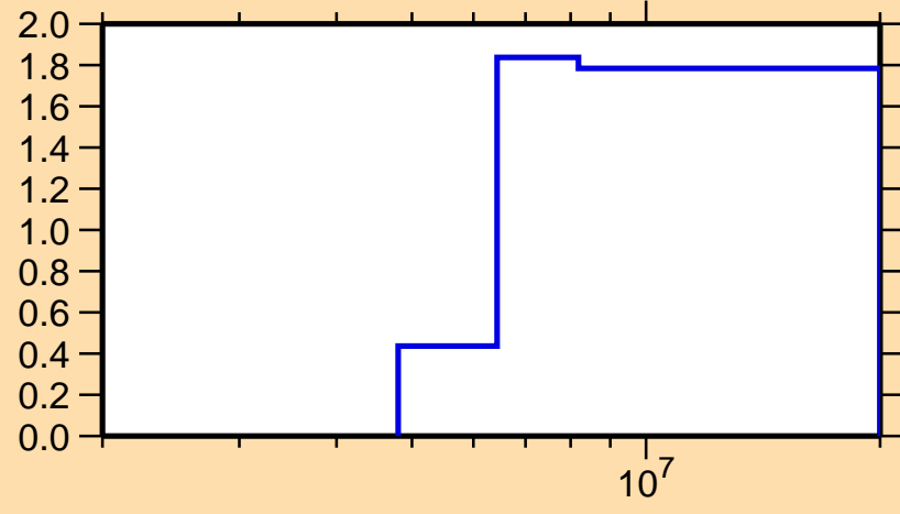
\sigma vs. E for ^{192}\text{Re}(n,2n)
