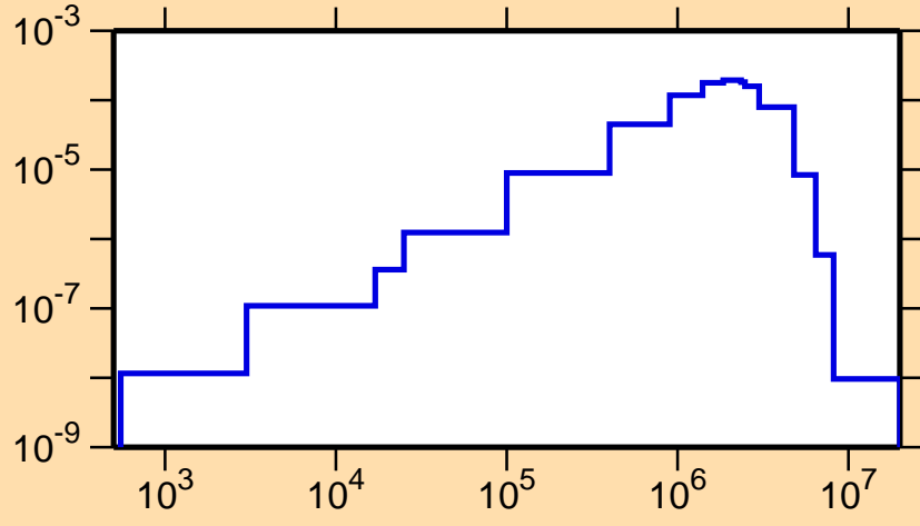
\sigma vs. E for ^{192}\text{Re}(n,n_1)
