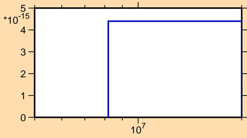
\sigma vs. E for ^{192}\text{Re}(n,\text{He3})
