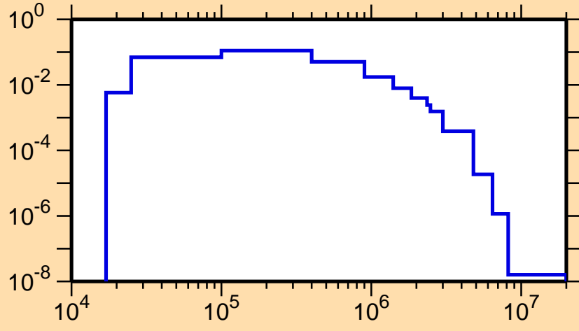
\sigma vs. E for ^{192}\text{Re}(n,n_3)
