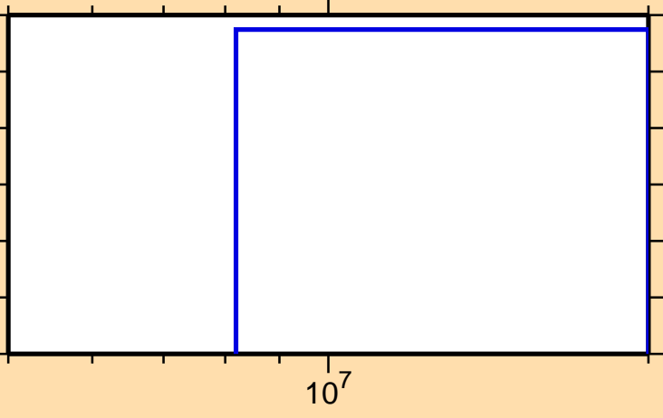
\sigma vs. E for ^{192}\text{Re}(n,nt)
