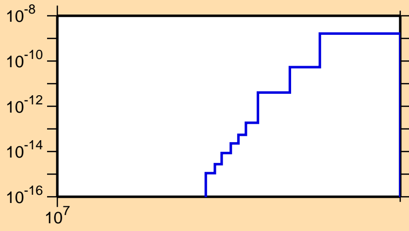
\sigma vs. E for ^{194}\text{Re}(n,2n\alpha)
