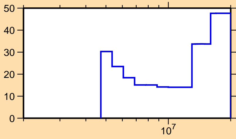
\Delta\sigma/\sigma vs. E for ^{194}\text{Re}(n,2n)
