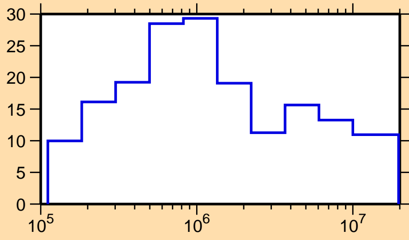
\Delta\sigma/\sigma vs. E for ^{195}\text{Re}(n, el.)
