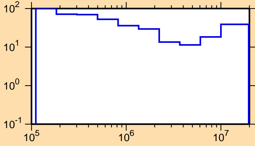
\Delta\sigma/\sigma vs. E for ^{195}\text{Re}(n,n\text{cont.})
