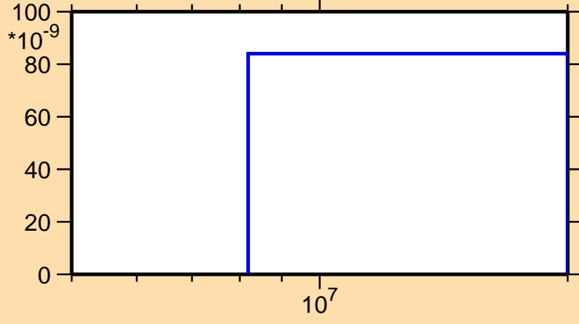
\sigma vs. E for ^{196}\text{Re}(n,n\alpha)
