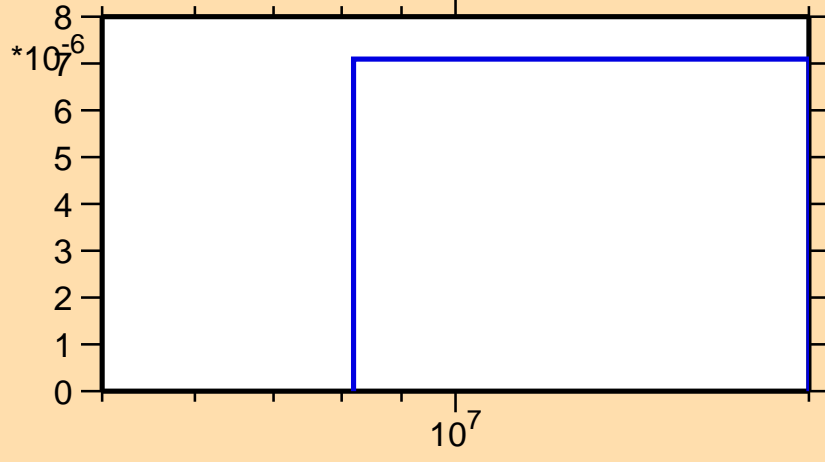
\sigma vs. E for ^{196}\text{Re}(n,t)
