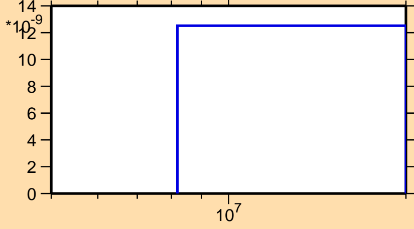
\sigma vs. E for ^{196}\text{Re}(n,nd)
