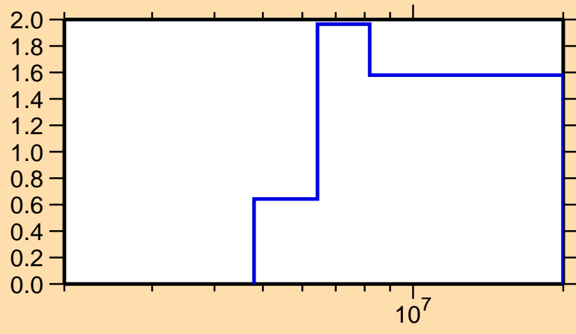
\sigma vs. E for ^{196}\text{Re}(n,2n)
