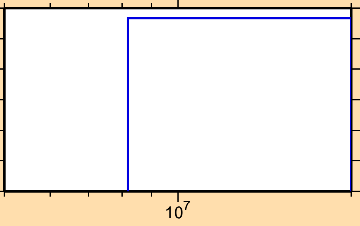
\sigma vs. E for ^{196}\text{Re}(n,2np)
