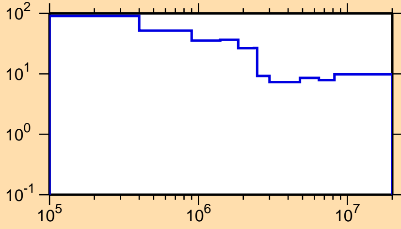
\Delta\sigma/\sigma vs. E for ^{196}\text{Re}(n,n\text{onel.})
