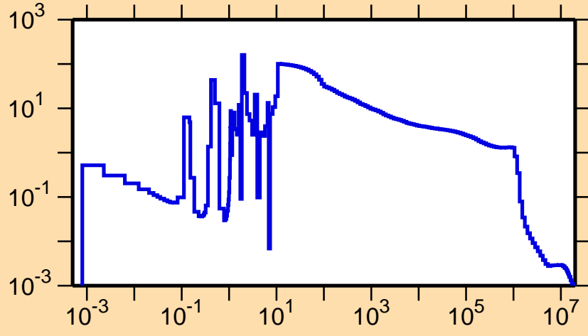
\sigma vs. E for ^{257}\gamma
