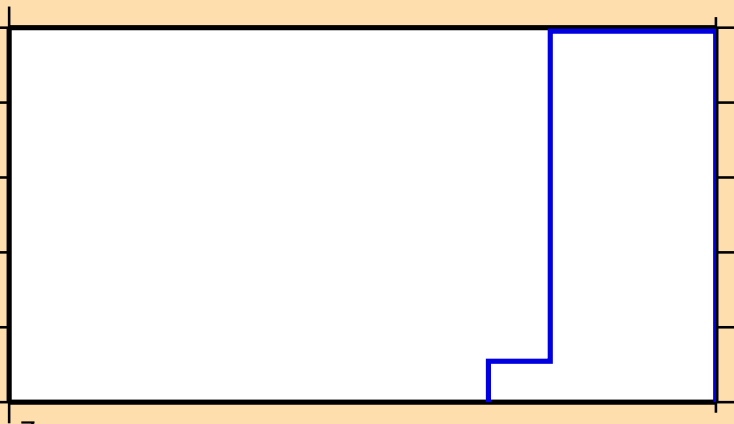
\sigma vs. E for ^{257}
