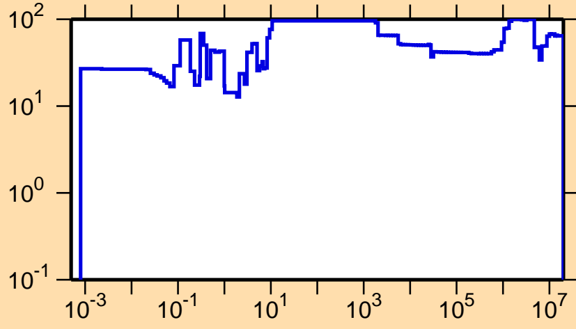
\Delta\sigma/\sigma vs. E for ^{257}\text{Pu}
