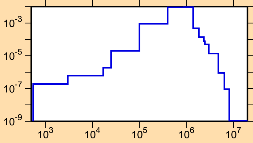
\sigma vs. E for ^{257}_{1}
