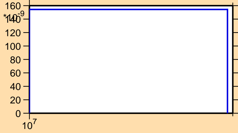
\sigma vs. E for ^{259}
