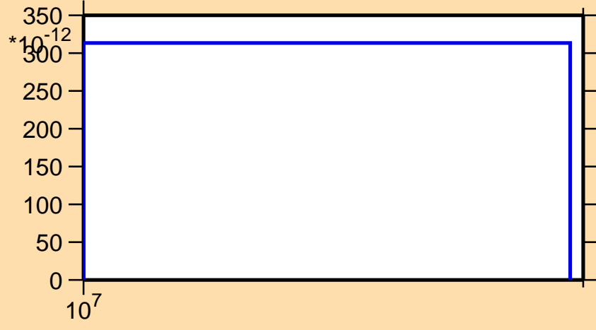
\sigma vs. E for ^{259}\alpha )
