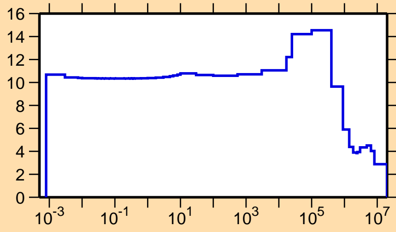
\sigma vs. E for ^{259}
