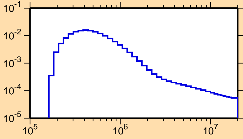
\sigma vs. E for ^{261}\text{Po}
