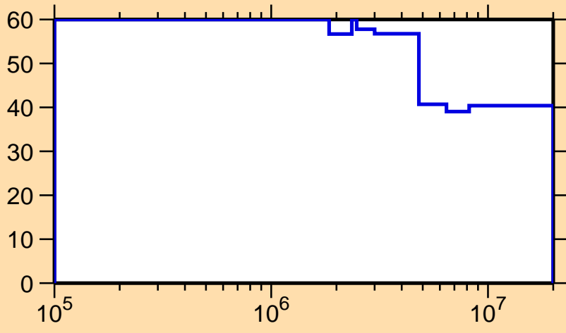
\Delta\sigma/\sigma vs. E for ^{261}_1
