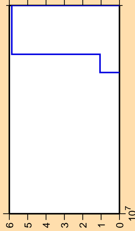
\Delta\sigma/\sigma vs. E for ^{261}
