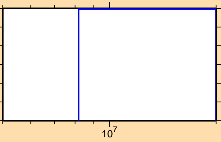
\sigma vs. E for ^{263}
