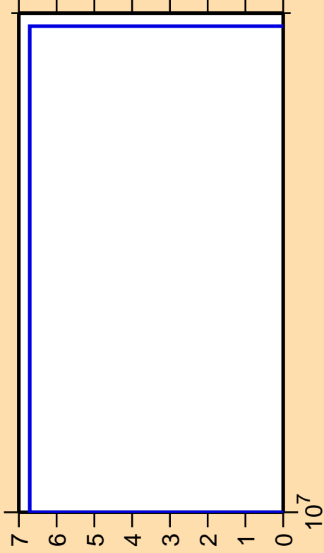
\Delta\sigma/\sigma vs. E for ^{264}\text{He3} )
