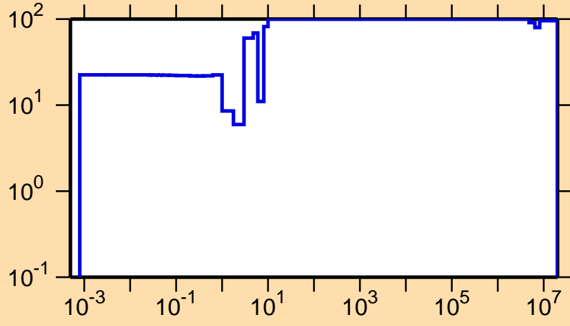
\Delta\sigma/\sigma vs. E for ^{264}\gamma
