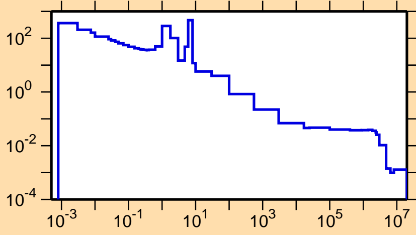
\sigma vs. E for ^{264}\gamma
