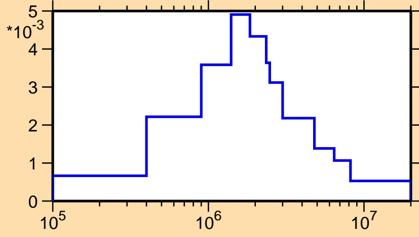
\sigma vs. E for ^{265}\text{Pu}
