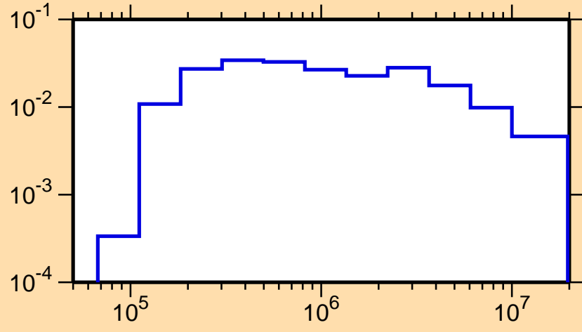
\sigma vs. E for ^{266}_{1}
