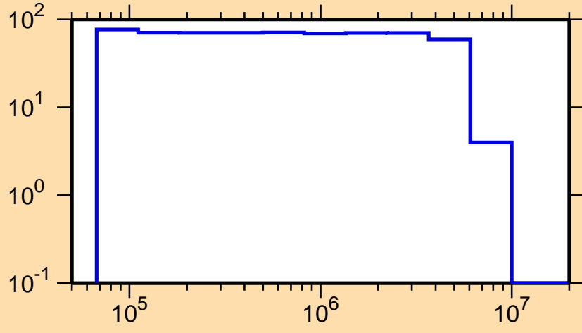
\Delta\sigma/\sigma vs. E for ^{280}_1
