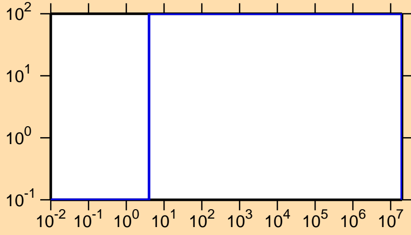
\Delta\sigma/\sigma vs. E for ^{282}\gamma
