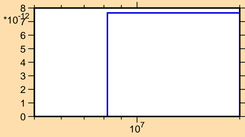
\sigma vs. E for ^{282}\text{He3}
