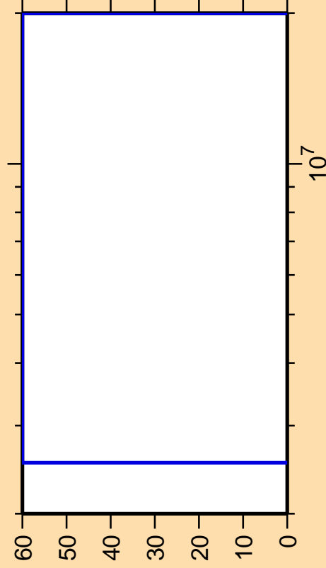
\Delta\sigma/\sigma vs. E for ^{283}\text{U}
