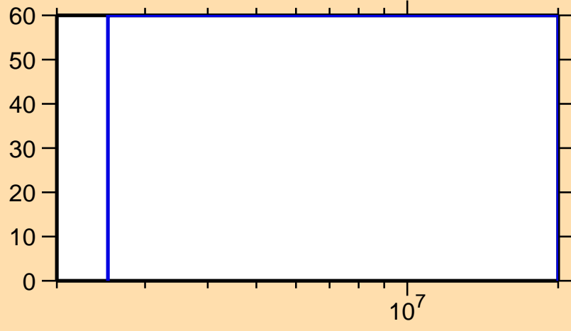
\Delta\sigma/\sigma vs. E for ^{283}\text{U}
