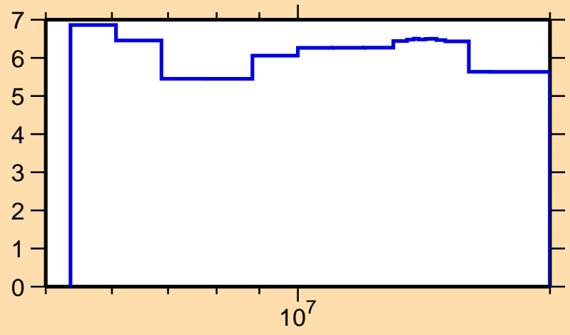
\Delta\sigma/\sigma vs. E for ^{91}\text{Rh}(n,n\text{onel.})
