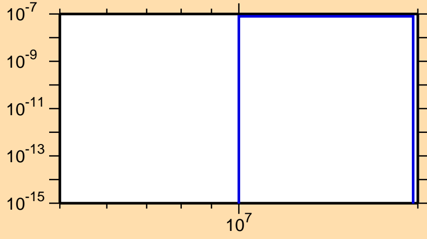
\sigma vs. E for ^{91}\text{Rh} (mt 45)
