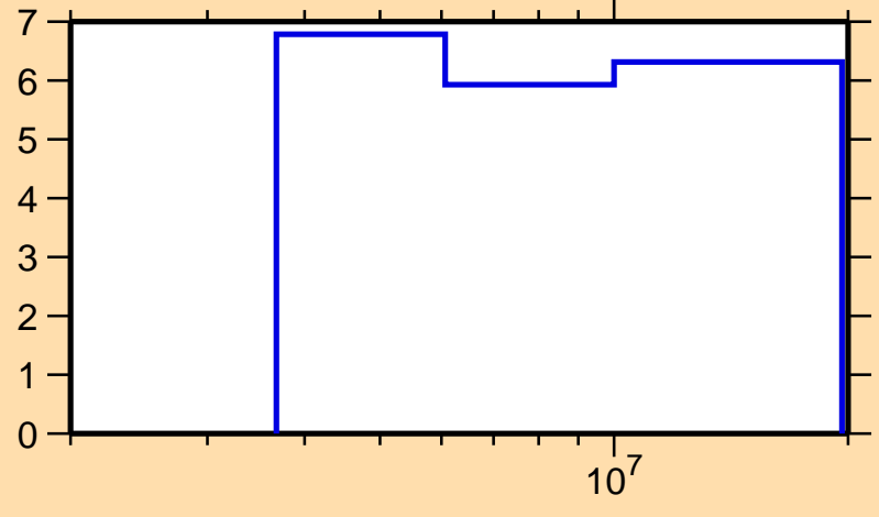
\Delta\sigma/\sigma vs. E for ^{91}\text{Rh}(n,n\text{nonel.})
