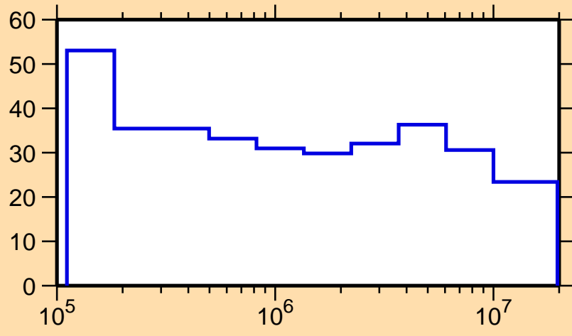
\Delta\sigma/\sigma vs. E for ^{91}\text{Rh}(n,n_1)
