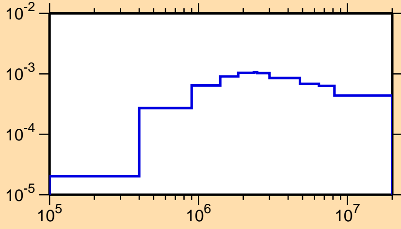
\sigma vs. E for ^{91}\text{Rh}(n,n_1)
